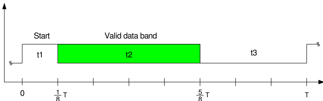
Figure 14 PWM format
