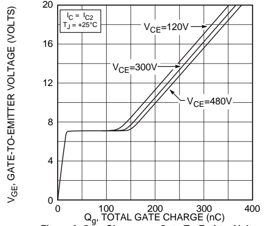
Figure 6, Gate Charges vs Gate-To-Emitter Voltage
