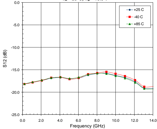
S12 versus Frequency, Over Temperature T_A = 25^\circ\text{C}, V_D = +3.9\text{ V}
