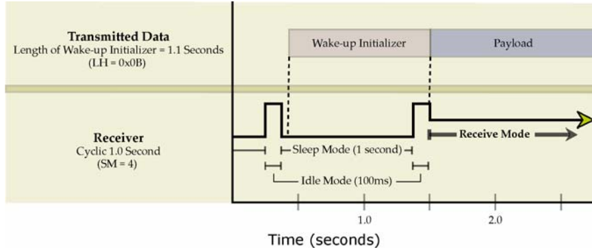
Figure 2-07. Incorrect Configuration (LH < SM)
