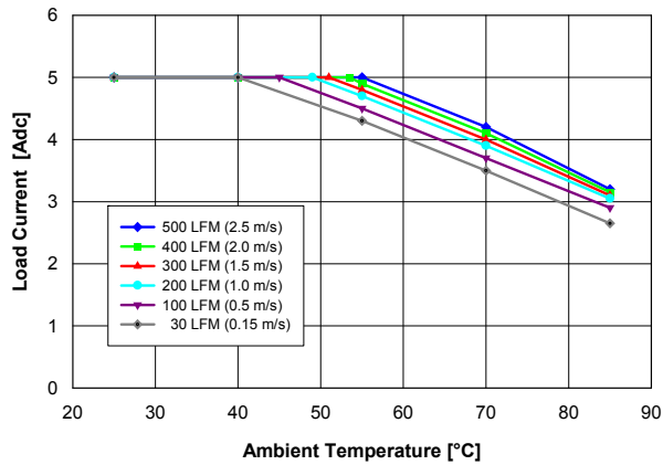
Fig. 5.0V.1: Available load current vs. ambient temperature and airflow rates for Vout = 5.0 V converter mounted vertically with Vin = 12 V, and maximum MOSFET temperature ≤ 120 °C.
