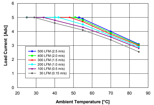
Fig. 5.0V.2: Available load current vs. ambient temperature and airflow rates for Vout = 5.0 V converter mounted horizontally with Vin = 12 V, and maximum MOSFET temperature ≤ 120 °C.
