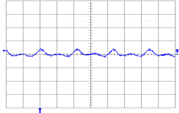
Fig. 2.5V.6: Output voltage ripple (20 mV/div.) at full rated load current into a resistive load with external capacitance 100 \mu\text{F} ceramic + 1 \mu\text{F} ceramic and V_{in} = 12 V for V_{out} = 2.5 V. Time scale: 2 \mu\text{s} /div.
