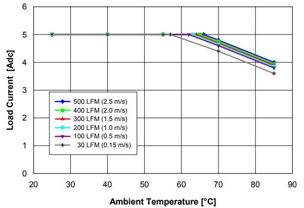
Fig. 1.2V.2: Available load current vs. ambient temperature and airflow rates for V out = 1.2 V converter mounted horizontally with V in = 12 V, and maximum MOSFET temperature ≤ 120 °C.
