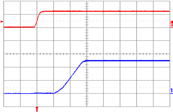
Fig. 2.5V.5: Turn-on transient for V_{out} = 2.5 V with application of V_{in} at full rated load current (resistive) and 100 \mu\text{F} external capacitance at V_{in} = 12 V. Top trace: V_{in} (10 V/div.); Bottom trace: output voltage (1 V/div.); Time scale: 5 ms/div.
