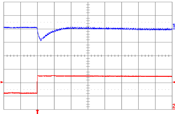
Fig. 2.5V.7: Output voltage response for V_{out} = 2.5 V to positive load current step change from 2.5 A to 5 A with slew rate of 5 \text{ A}/\mu\text{s} at V_{in} = 12 V. Top trace: output voltage (100 mV/div.); Bottom trace: load current (2 A/div.). C_o = 100 \mu\text{F} ceramic. Time scale: 20 \mu\text{s} /div.
