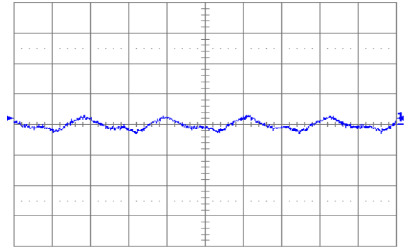
Fig. 5.0V.6: Output voltage ripple (20 mV/div.) at full rated load current into a resistive load with external capacitance 100 \mu\text{F} ceramic and V_{in} = 12 V for V_{out} = 5.0 V. Time scale: 1 \mu\text{s} /div.
