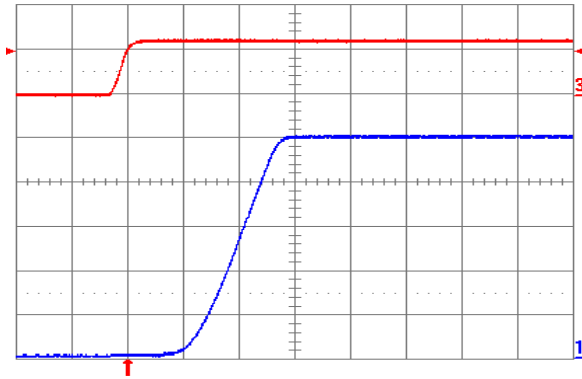
Fig. 5.0V.5: Turn-on transient for V_{out} = 5.0 V with application of V_{in} at full rated load current (resistive) and 100 \mu\text{F} external capacitance at V_{in} = 12 V. Top trace: V_{in} (10 V/div.); Bottom trace: output voltage (1 V/div.); Time scale: 5 ms/div.
