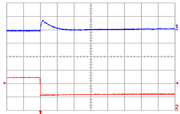
Fig. 2.5V.8: Output voltage response for V_{out} = 2.5 V to negative load current step change from 5 A to 2.5 A with slew rate of -5 \text{ A}/\mu\text{s} at V_{in} = 12 V. Top trace: output voltage (100 mV/div.); Bottom trace: load current (2 A/div.). C_o = 100 \mu\text{F} ceramic. Time scale: 20 \mu\text{s} /div.
