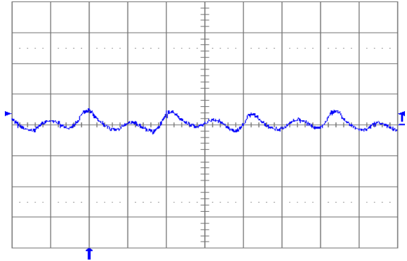
Fig. 1.5V.6: Output voltage ripple (20 mV/div.) at full rated load current into a resistive load with external capacitance 100\ \mu\text{F} ceramic and V_{in} = 12\text{ V} for V_{out} = 1.5\text{ V} . Time scale: 1 \mu\text{s} /div.
