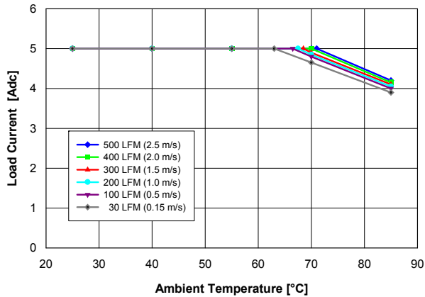
Fig. 0.7525V.1: Available load current vs. ambient temperature and airflow rates for Vout = 0.7525 V converter mounted vertically with Vin = 12 V, and maximum MOSFET temperature ≤ 120 °C.
