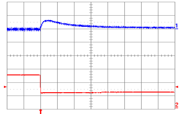
Fig. 0.7525V.8: Output voltage response for V_{out} = 0.7525\text{V} to negative load current step change from 5 A to 2.5 A with slew rate of -5\ \text{A}/\mu\text{s} at V_{in} = 12\ \text{V} . Top trace: output voltage (100 mV/div.); Bottom trace: load current (2 A/div.). C_o = 100\ \mu\text{F} ceramic. Time scale: 20 \mu\text{s} /div.
