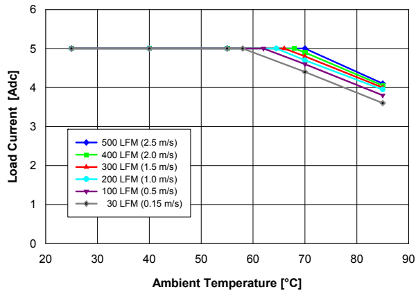
Fig. 1.2V.1: Available load current vs. ambient temperature and airflow rates for V out = 1.2 V converter mounted vertically with V in = 12 V, and maximum MOSFET temperature ≤ 120 °C.
