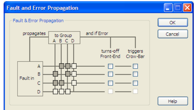
Figure 42. Fault and Error Propagation Window
