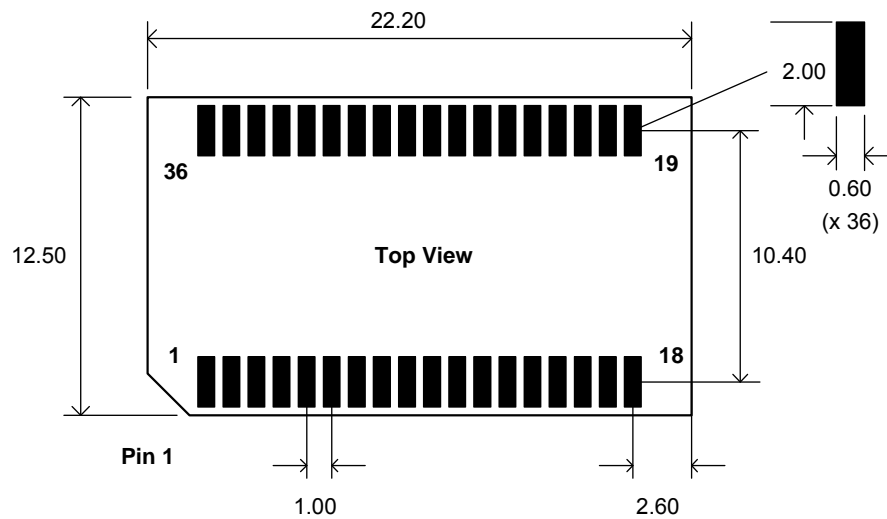
Figure 59. Recommended PCB Pad Sizes
