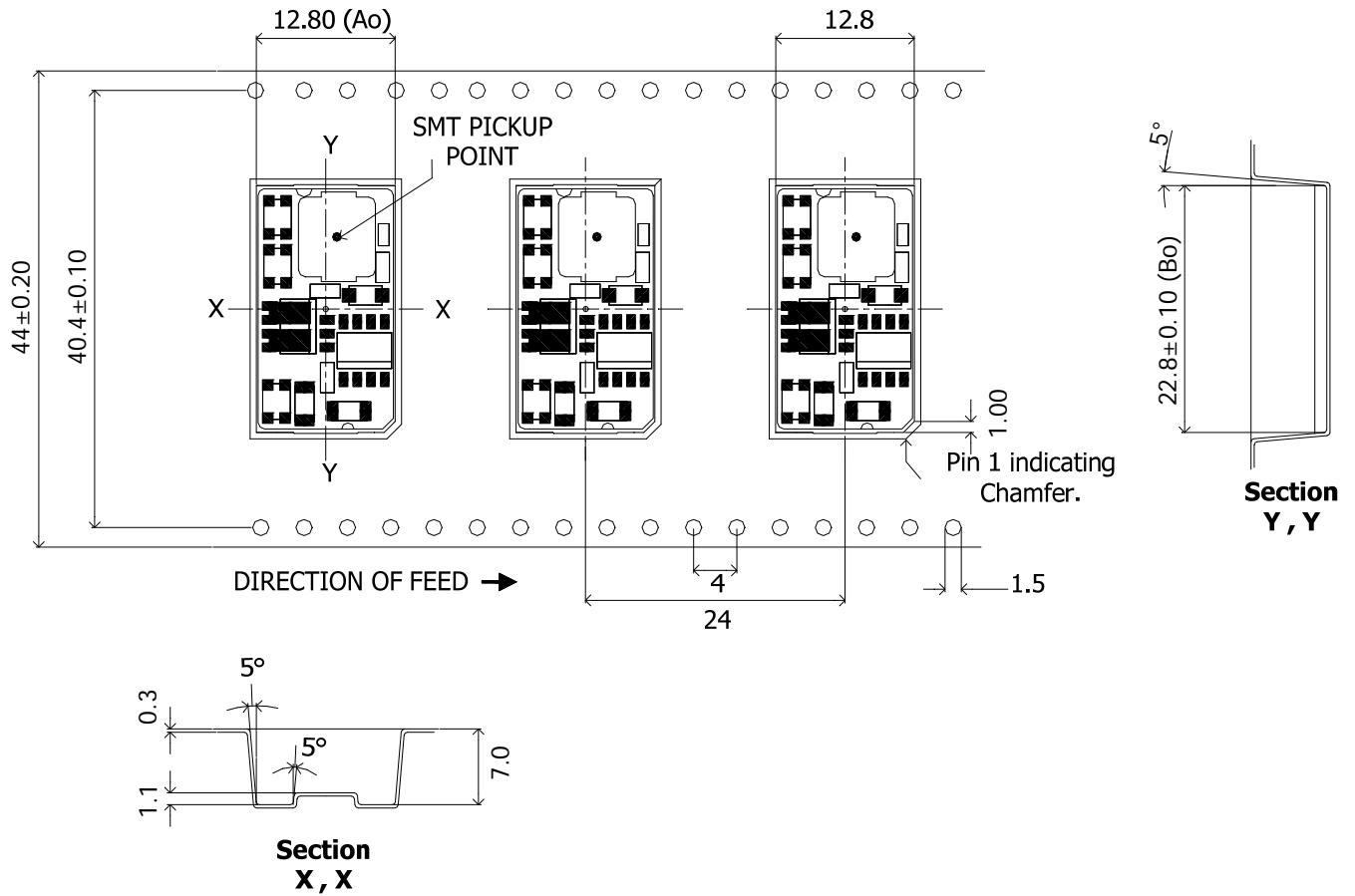
Figure 58. Tape and Reel
