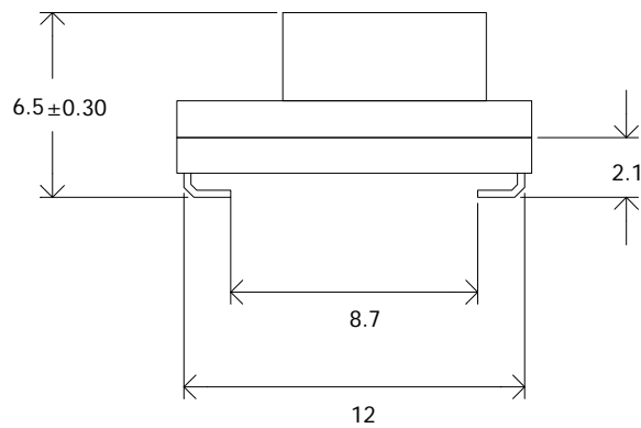
Figure 57. Side View
