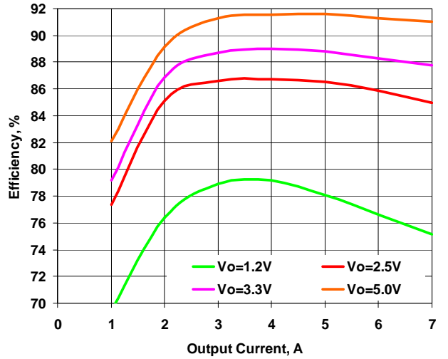
Figure 5. Efficiency vs. Load. Vin=12V, Fsw=500kHz
