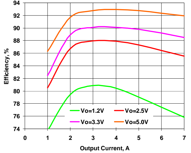
Figure 4. Efficiency vs. Load. Vin=9.6V, Fsw=500kHz
