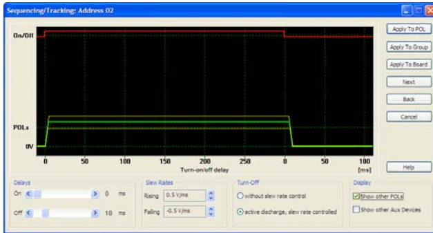
Figure 30. Sequencing/Tracking Window
