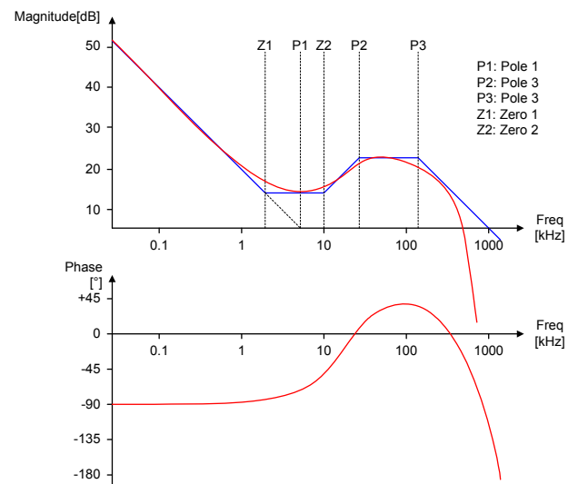
Figure 52. Transfer Function of PWM
