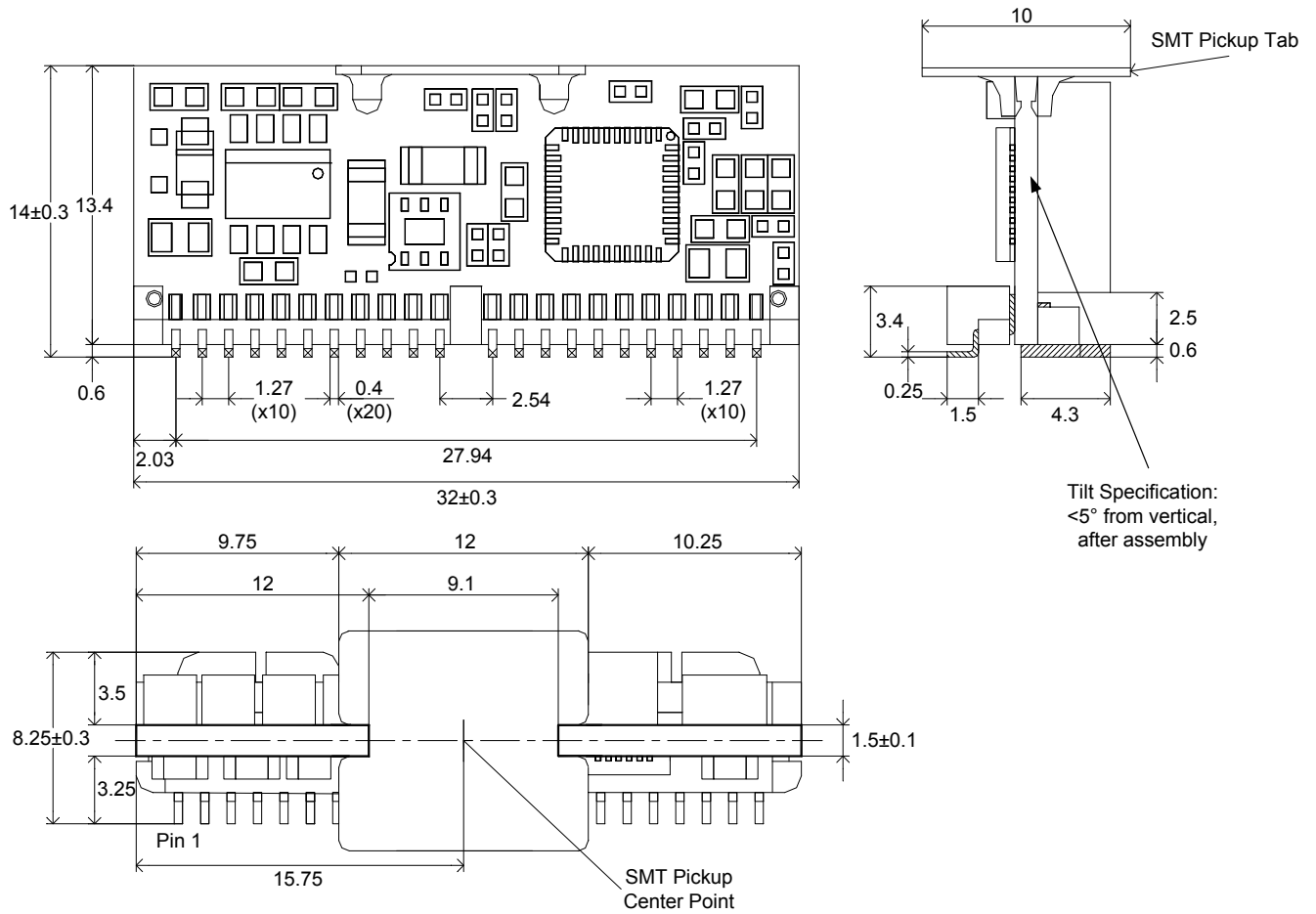
Figure 20. Mechanical Drawing
