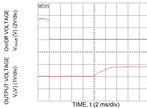
Figure 17. Typical Start-Up with Prebias ( V_{in} = 3.3\text{ Vdc} , V_o = 1.8\text{ Vdc} , I_o = 1\text{ A} , V_{bias} = 1.0\text{ Vdc} ).
