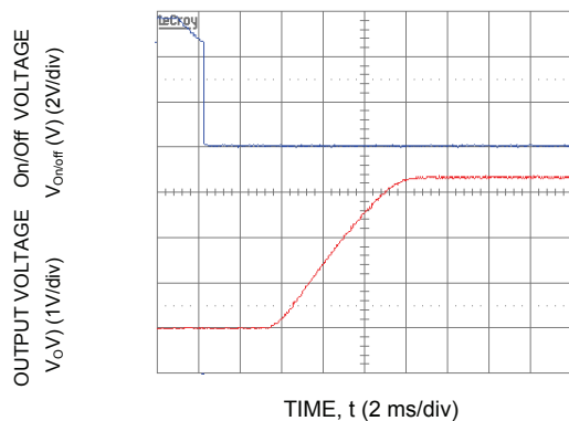
Figure 15. Typical Start-Up Using Remote On/Off with external capacitors ( V_{in} = 5.5\text{ Vdc} , V_o = 3.3\text{ Vdc} , I_o = 10\text{ A} , C_o = 1050\ \mu\text{F} ).
