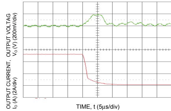
Figure 11. Transient Response to Dynamic Load Change from 100% to 50% of full load ( V_o = 5.0 Vdc ).
