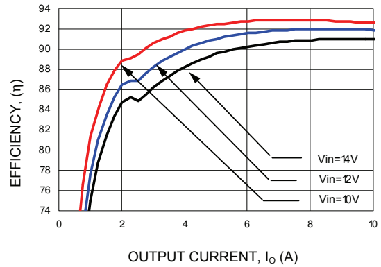
Figure 4. Converter Efficiency versus Output Current (Vout = 2.5Vdc).
