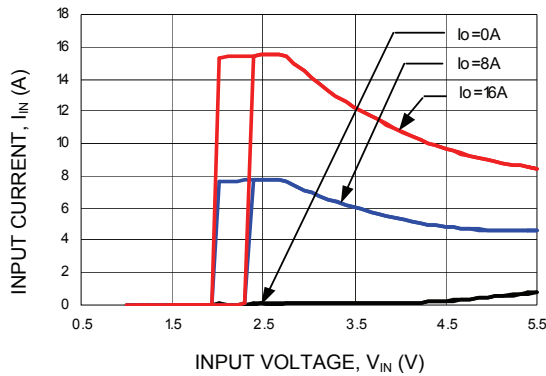
Figure 7. Input voltage vs. Input Current (V out = 2.5Vdc).
