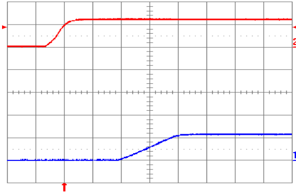
Fig. 1.2V.4: Turn-on transient for V_{out} = 1.2\text{ V} with application of V_{in} at full rated load current (resistive) and 100\ \mu\text{F} external capacitance at V_{in} = 12\text{ V} . Top trace: V_{in} (10V/div.); Bottom trace: output voltage (1 V/div.); Time scale: 2 ms/div.
