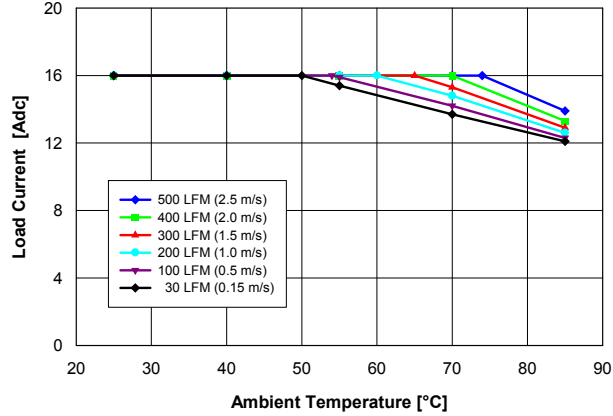
Fig. 1.8V.1: Available load current vs. ambient temperature and airflow rates for V out = 1.8 V converter mounted vertically with V in = 12 V, and maximum MOSFET temperature ≤ 120 °C.
