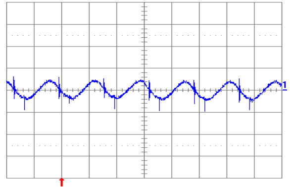
Fig. 2.5V.5: Output voltage ripple (20 mV/div.) at full rated load current into a resistive load with external capacitance 100\ \mu\text{F} ceramic and V_{in} = 12\text{ V} for V_{out} = 2.5\text{ V} . Time scale: 2 \mu\text{s} /div.
