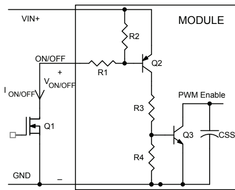
Figure 28. Remote On/Off Implementation.
