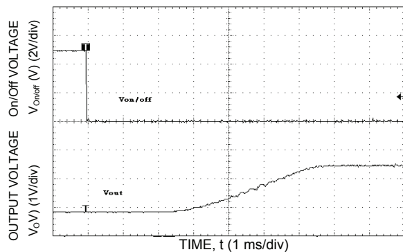
Figure 15. Typical Start-Up Using Remote On/Off with Low-ESR external capacitors ( 7 \times 150\ \mu\text{F} Polymer) ( V_{in} = 12\text{ Vdc} , V_o = 3.3\text{ Vdc} , I_o = 6.0\text{ A} , C_o = 1050\ \mu\text{F} ).
