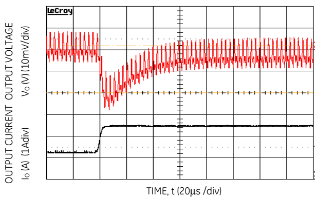
Figure 4. Transient Response to Dynamic Load Change from 50% to 100% at 28Vin, C_{ext} = 10\mu F ceramic + 330 \mu F polymer, C_{Tune} = 5600pF & R_{Tune} = 261\Omega
