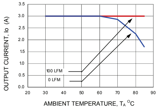
Figure 22. Derating Output Current versus Local Ambient Temperature and Airflow ( V_{IN} = 12 \text{ Vdc} , V_o=5.0 \text{ Vdc} ).
