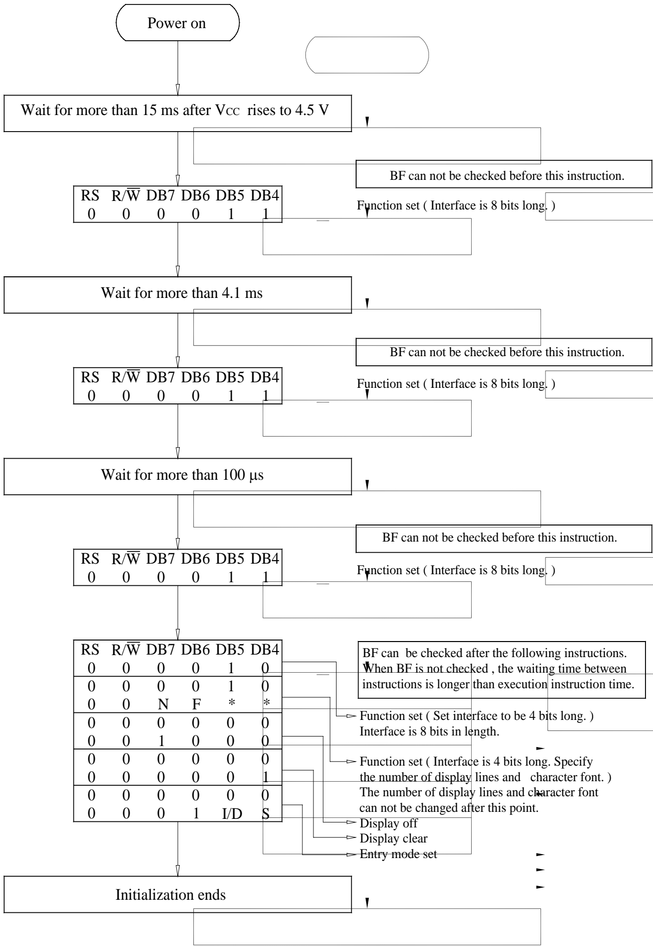
4-Bit Inerface
