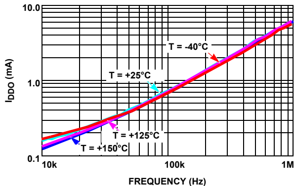
FIGURE 3. HIP2122 I_{DDQ} OPERATING CURRENT vs FREQUENCY
