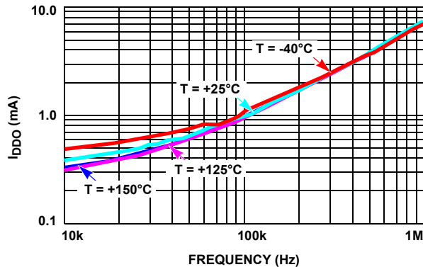
FIGURE 4. HIP2123 I_{DDQ} OPERATING CURRENT vs FREQUENCY
