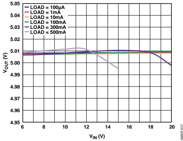
Figure 17. Output Voltage vs. Input Voltage, V_{OUT} = 5V
