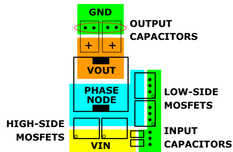
FIGURE 12. TYPICAL POWER COMPONENT PLACEMENT
