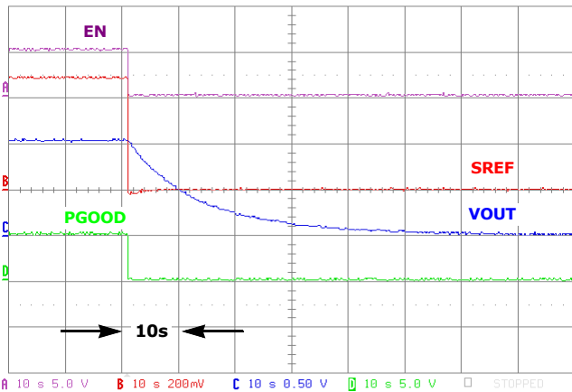
FIGURE 19. SHUT-DOWN, V_{IN} = 12.6V , V_{OUT} = 1.05V , LOAD = OPEN-CIRCUIT
