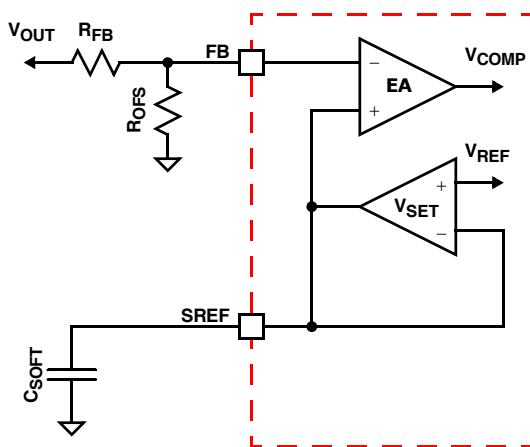
FIGURE 4. ISL78210 VOLTAGE PROGRAMMING
