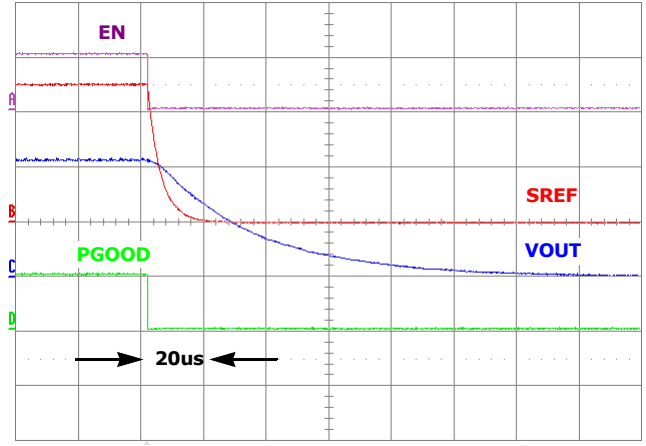
FIGURE 18. SHUT-DOWN, V_{IN} = 12.6V , V_{OUT} = 1.05V , LOAD = 50m \Omega
