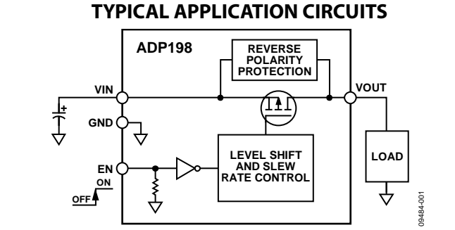
Figure 1. WLCSP
