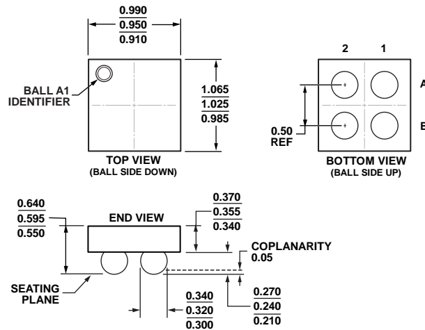
Figure 33. 4-Ball Wafer Level Chip Scale Package [WLCSP] (CB-4-4) Dimensions shown in millimeters
