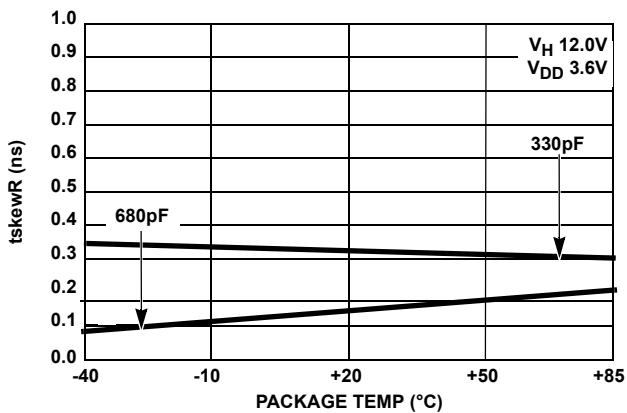
FIGURE 27. tSkewR vs TEMPERATURE
