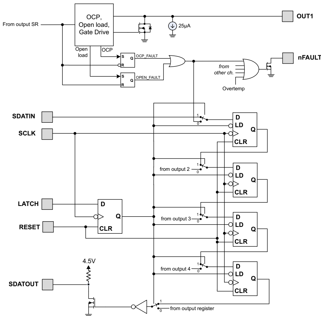
Figure 3. Fault Output
