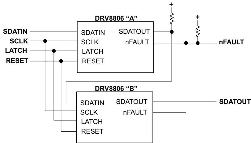
Figure 4. Daisy-Chain Connection
