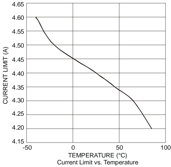
Current Limit vs. Temperature
