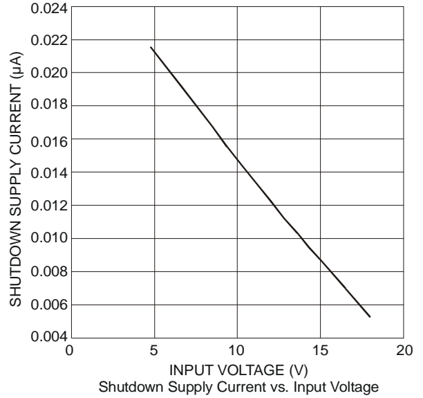
Shutdown Supply Current vs. Input Voltage
