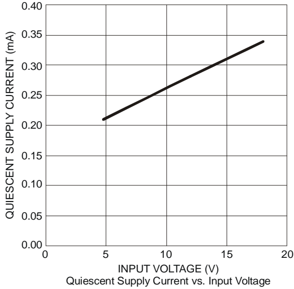
Quiescent Supply Current vs. Input Voltage
