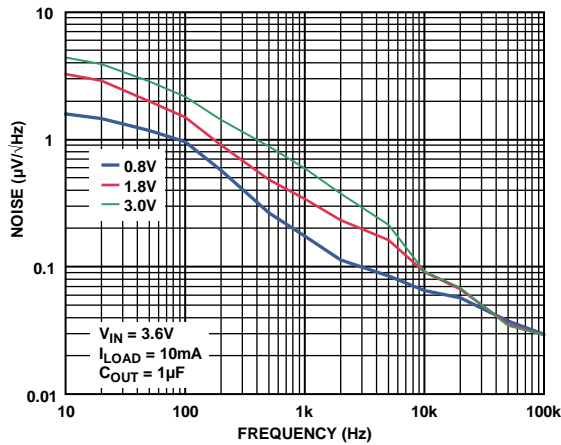
Figure 17. Output Noise Spectrum
