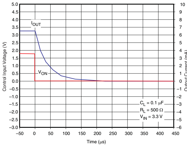
Figure 22. t_{ON} Response
