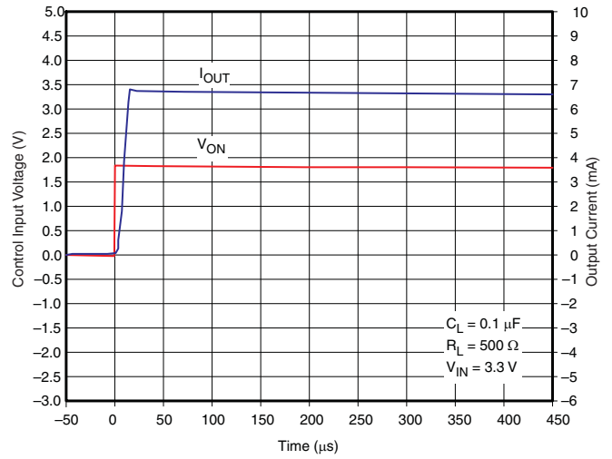
Figure 21. t_{ON} Response
