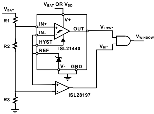
FIGURE 27. WINDOW COMPARATOR CIRCUIT
