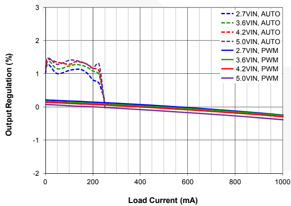
Figure 8. \Delta V_{OUT} (%) vs. Load Current and Input Voltage, Normalized to 3.6\text{ V}_{IN} , 500 mA Load, FPWM, Dotted for Auto Mode
