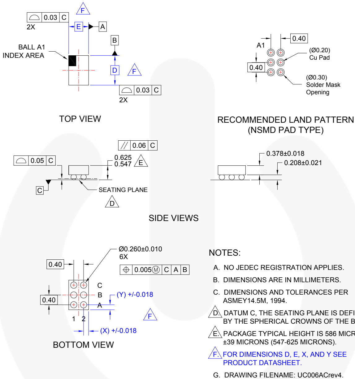
Figure 1. 6-Bump WLCSP, 0.4 mm Pitch
