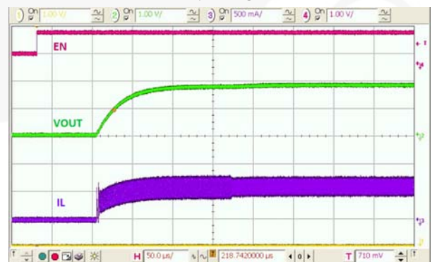
Figure 23. Startup, 3 \Omega Load
