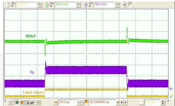
Figure 17. Load Transient, 200-800-200 mA, 100 ns Edge
