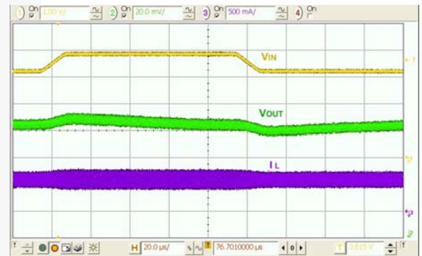
Figure 19. Line Transient, 3.3-3.9-3.3 V_{IN} , 10 \mu\text{s} Edge, 600 mA Load
