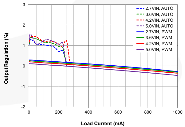
Figure 9. \Delta V_{OUT} (%) vs. Load Current and Input Voltage, V_{OUT} = 1.23\text{ V} , Normalized to 3.6\text{ V}_{IN} , 500 mA Load, FPWM, Dotted for Auto Mode
