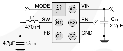
Figure 1. Typical Application
