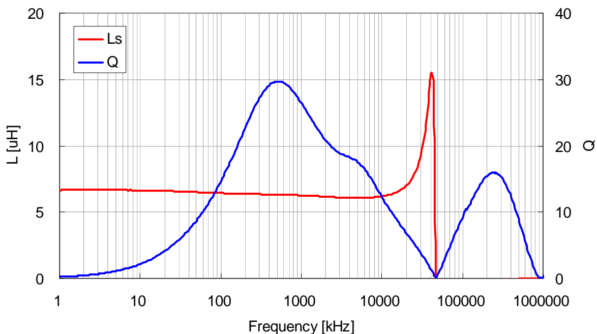
VLS3012T-6R8MR90
