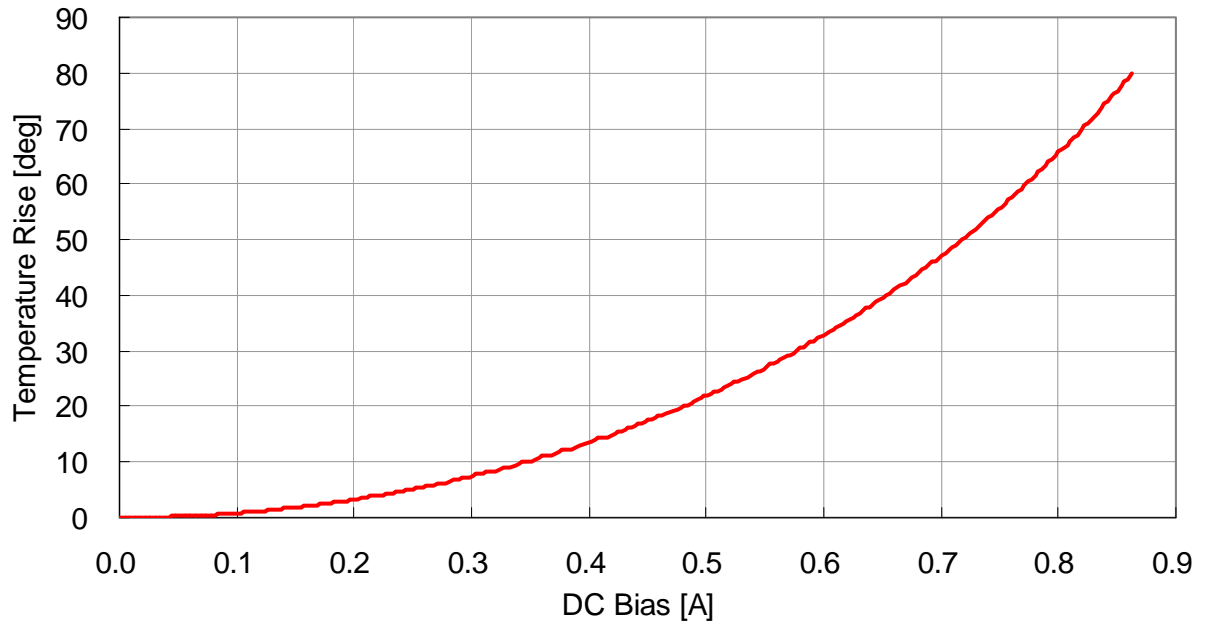
VLS3012T-330MR40
