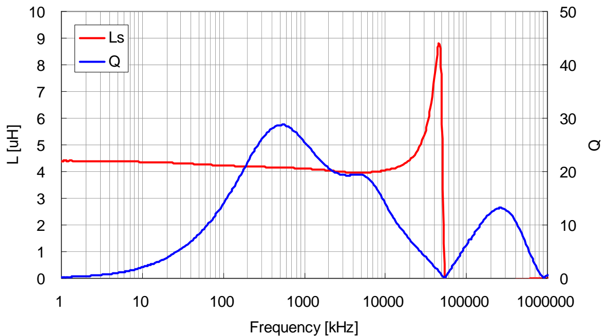
VLS3012T-4R7M1R0
